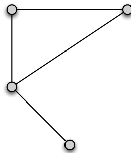
H_3 \subseteq G , induciran.
