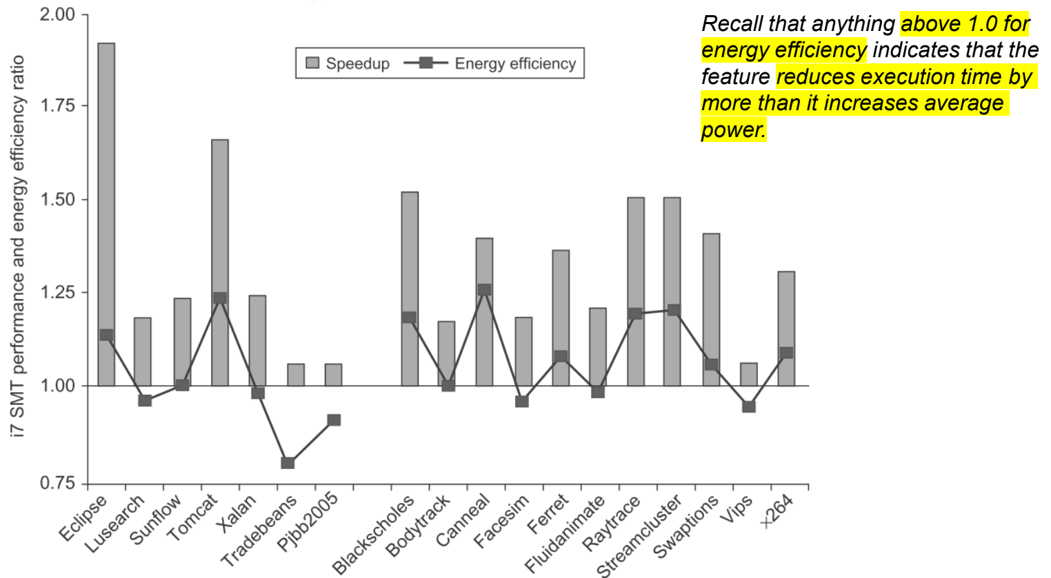
Figure 3.33: The speedup from using multithreading on one core on an i7 processor averages 1.28 for the Java benchmarks and 1.31 for the PARSEC benchmarks
