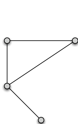
H_3 \subseteq G , induciran.
