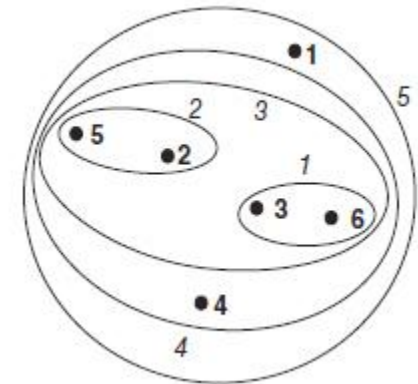
single link
