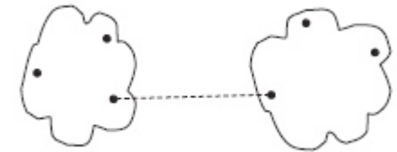
single link
