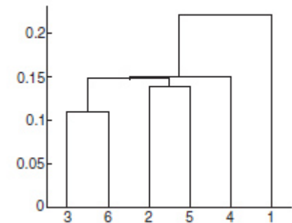
single link
